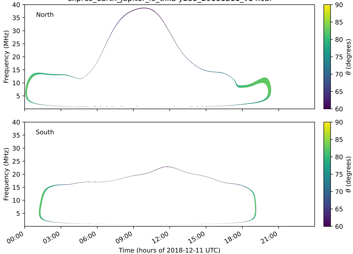
expres_earth_jupiter_io_txka-y235_20181211_v14.cdf
