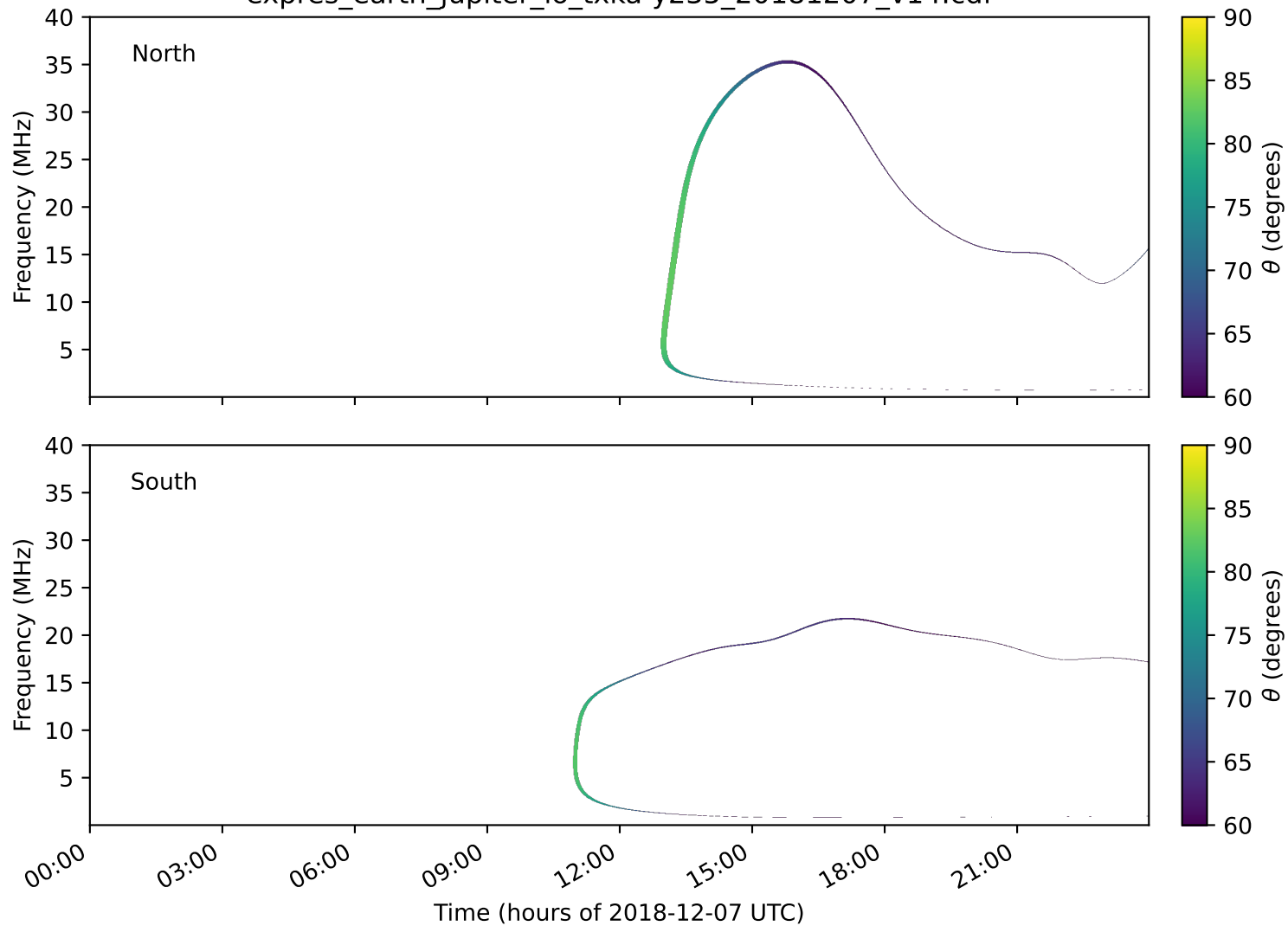
expres_earth_jupiter_io_txka-y235_20181207_v14.cdf
