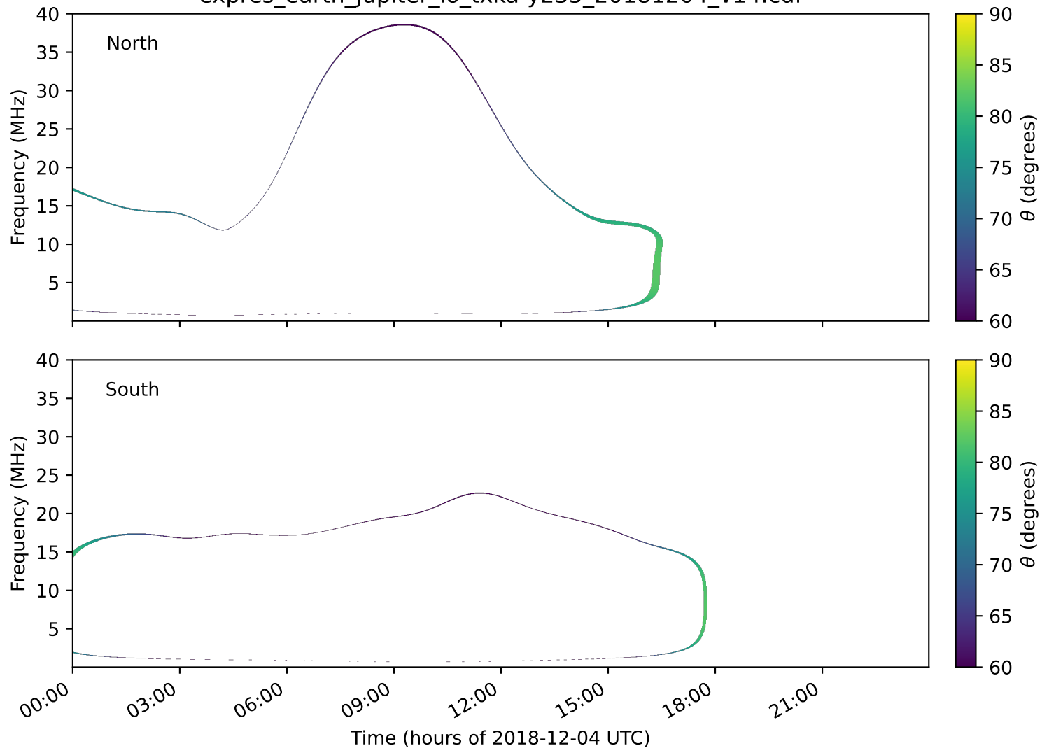
expres_earth_jupiter_io_txka-y235_20181204_v14.cdf
