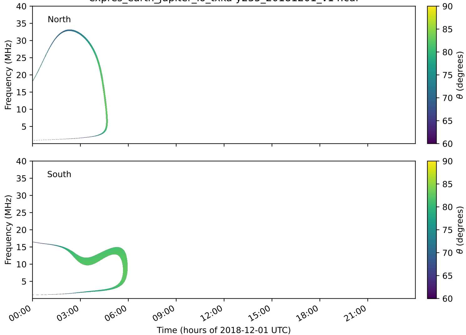
expres_earth_jupiter_io_txka-y235_20181201_v14.cdf
