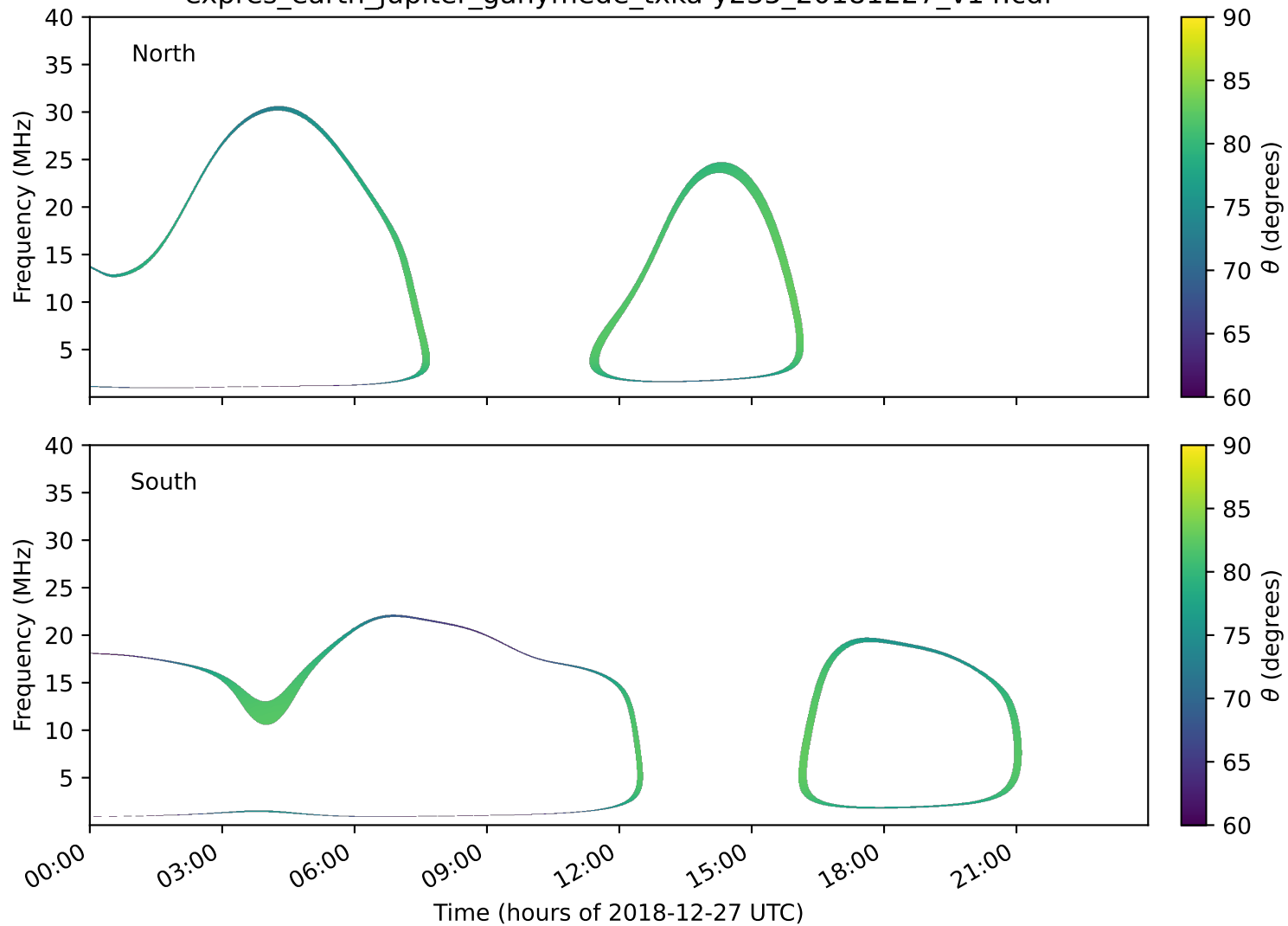
expres_earth_jupiter_ganymede_txka-y235_20181227_v14.cdf
