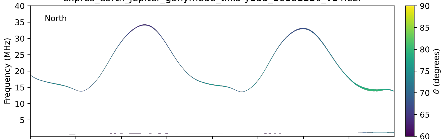
expres_earth_jupiter_ganymede_txka-y235_20181226_v14.cdf
