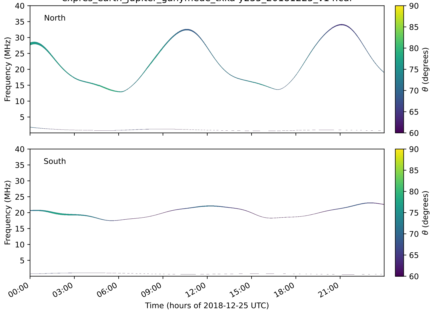
expres_earth_jupiter_ganymede_txka-y235_20181225_v14.cdf
