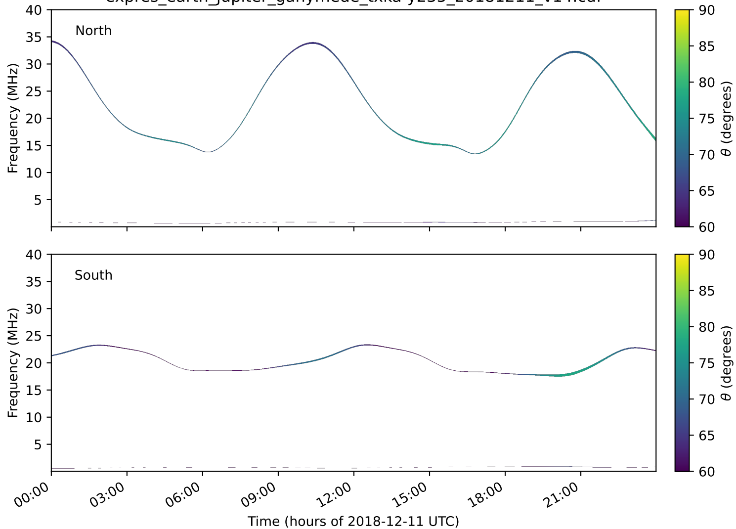
expres_earth_jupiter_ganymede_txka-y235_20181211_v14.cdf
