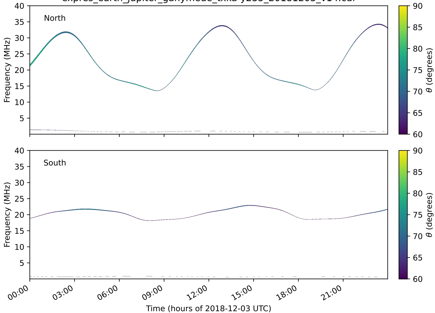
expres_earth_jupiter_ganymede_txka-y235_20181203_v14.cdf
