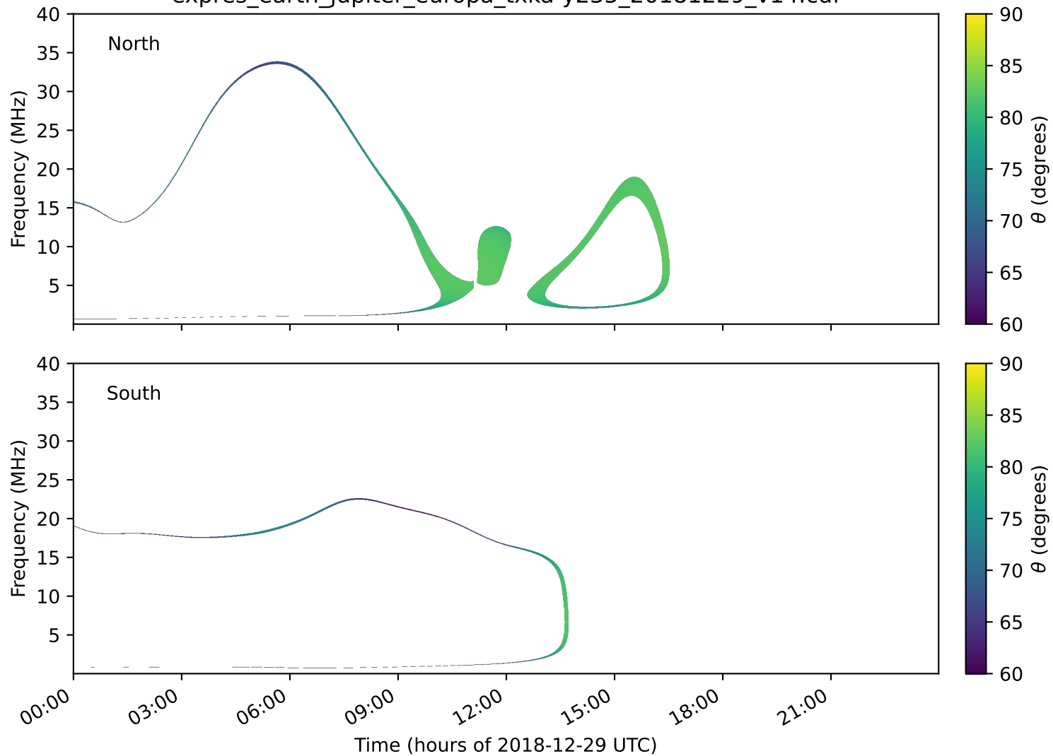
expres_earth_jupiter_europa_txka-y235_20181229_v14.cdf
