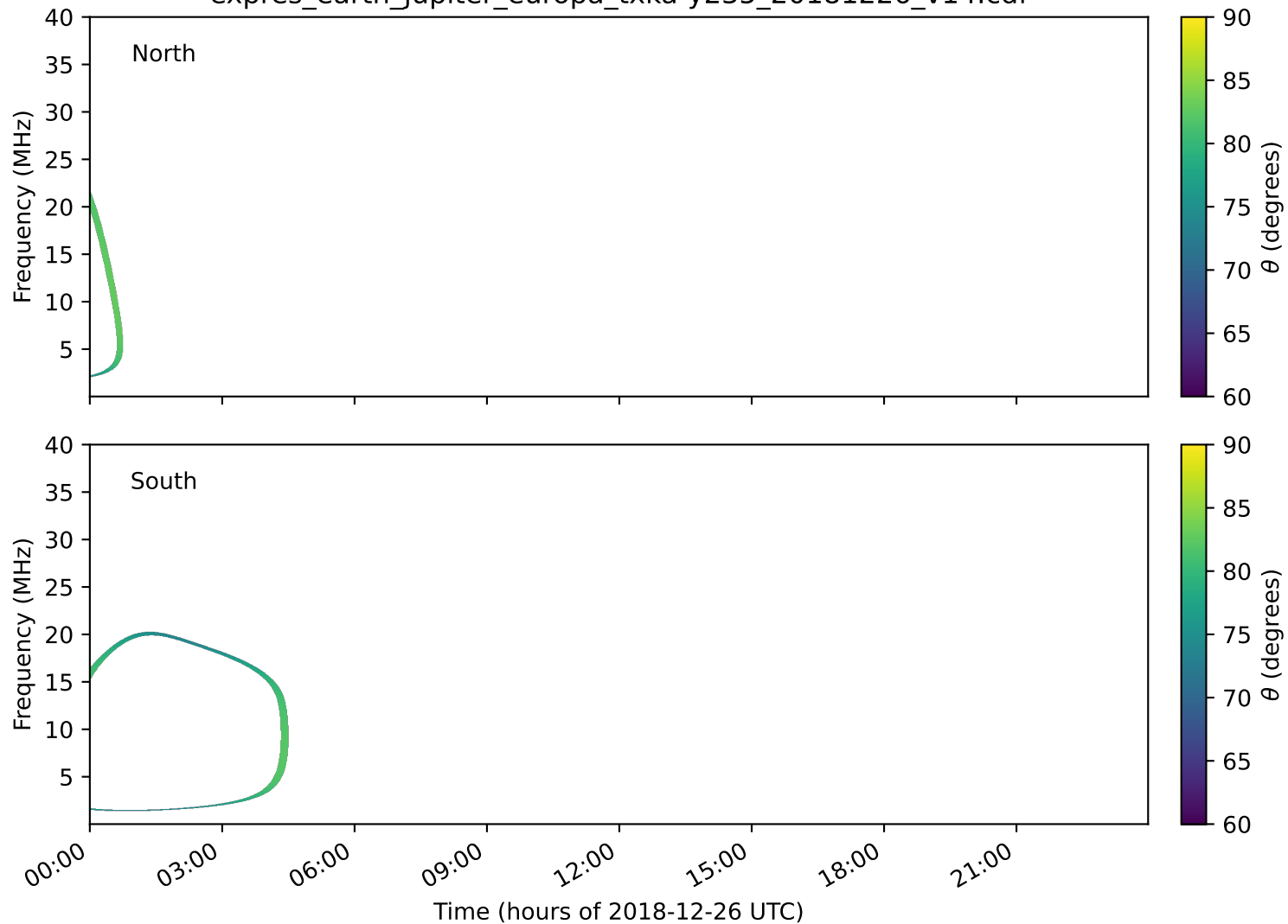
expres_earth_jupiter_europa_txka-y235_20181226_v14.cdf
