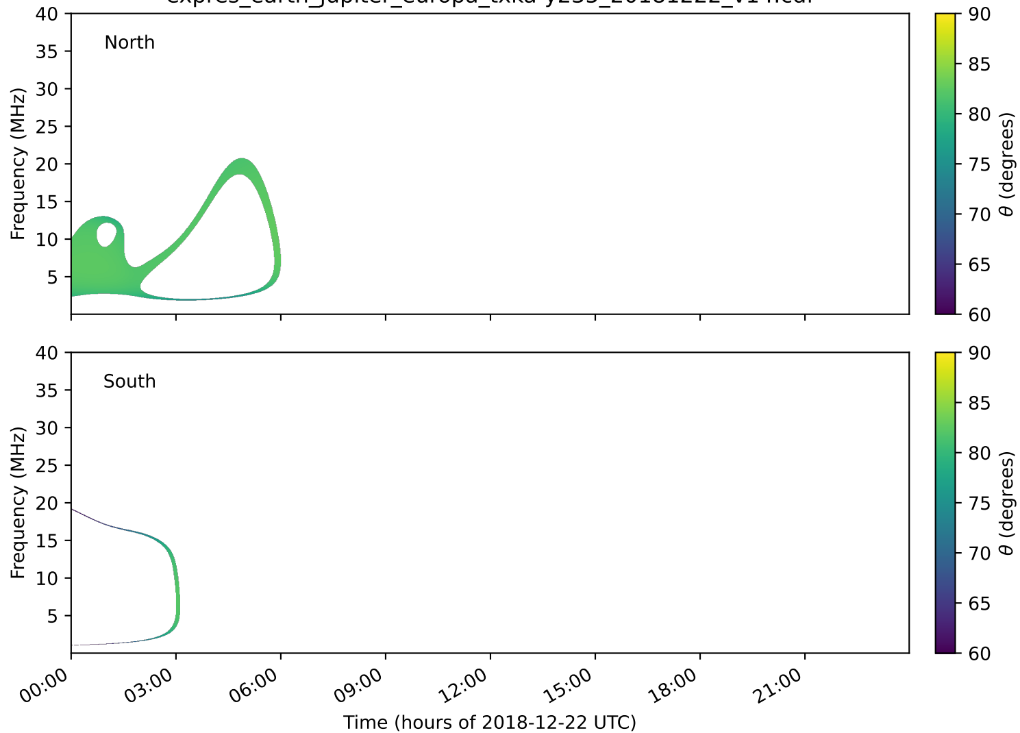
expres_earth_jupiter_europa_txka-y235_20181222_v14.cdf
