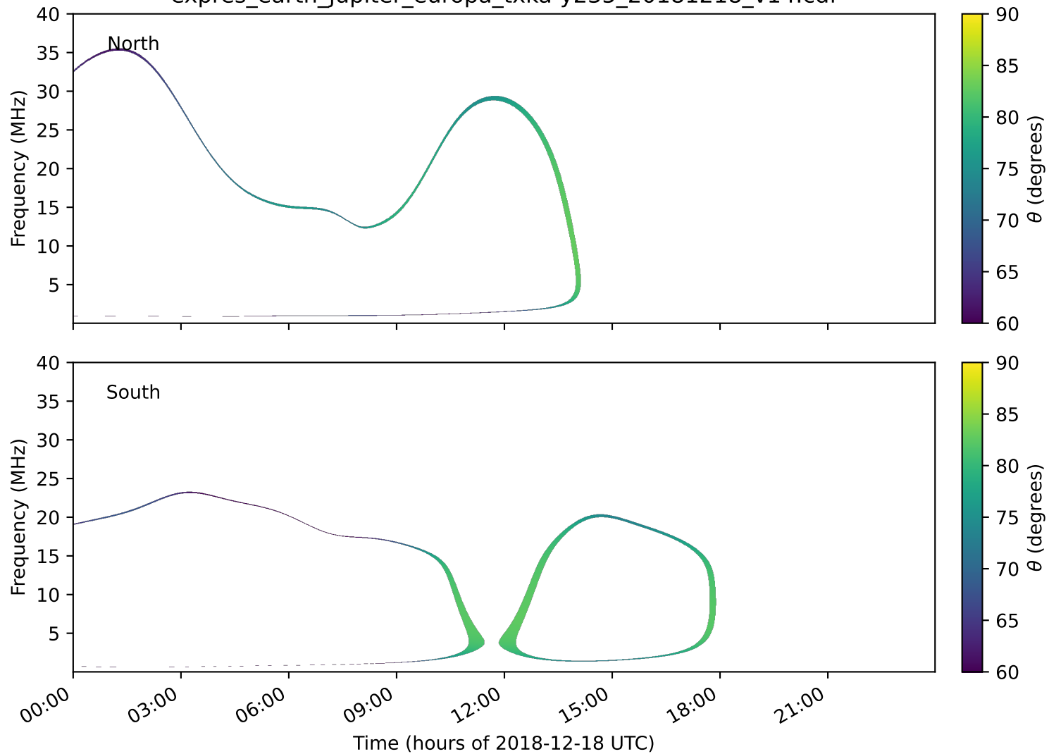
expres_earth_jupiter_europa_txka-y235_20181218_v14.cdf
