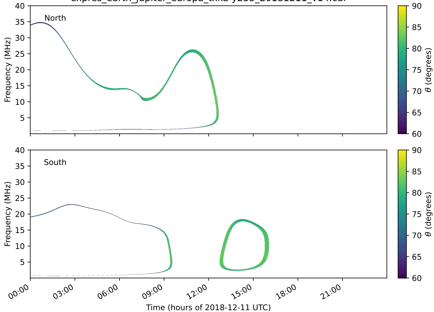
expres_earth_jupiter_europa_txka-y235_20181211_v14.cdf
