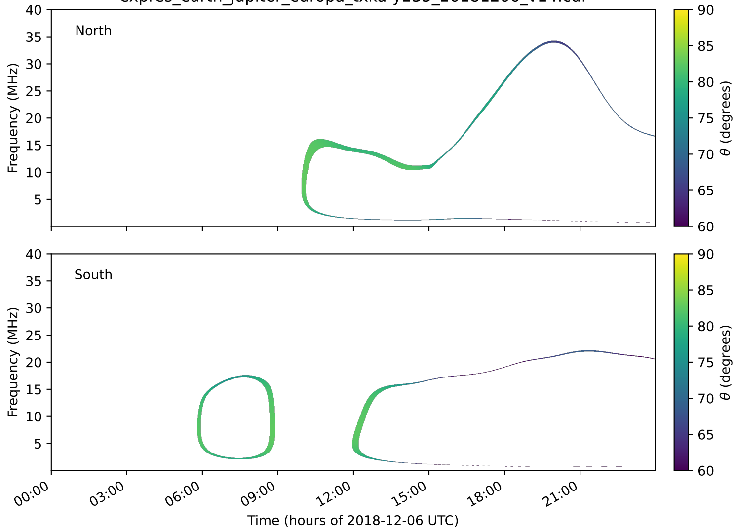
expres_earth_jupiter_europa_txka-y235_20181206_v14.cdf
