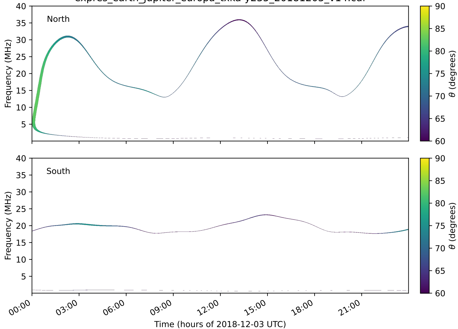
expres_earth_jupiter_europa_txka-y235_20181203_v14.cdf
