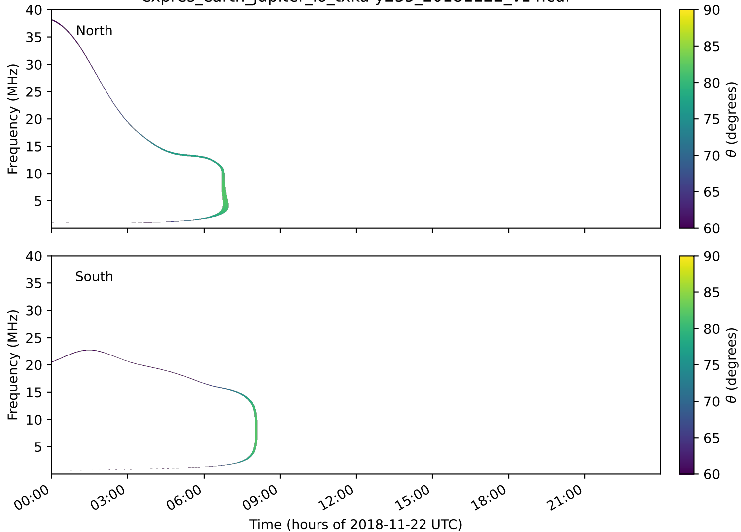
expres_earth_jupiter_io_txka-y235_20181122_v14.cdf
