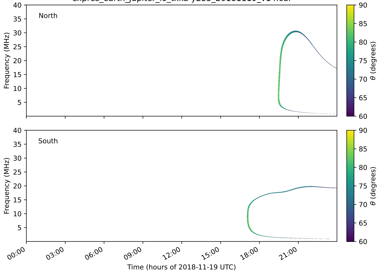
expres_earth_jupiter_io_txka-y235_20181119_v14.cdf
