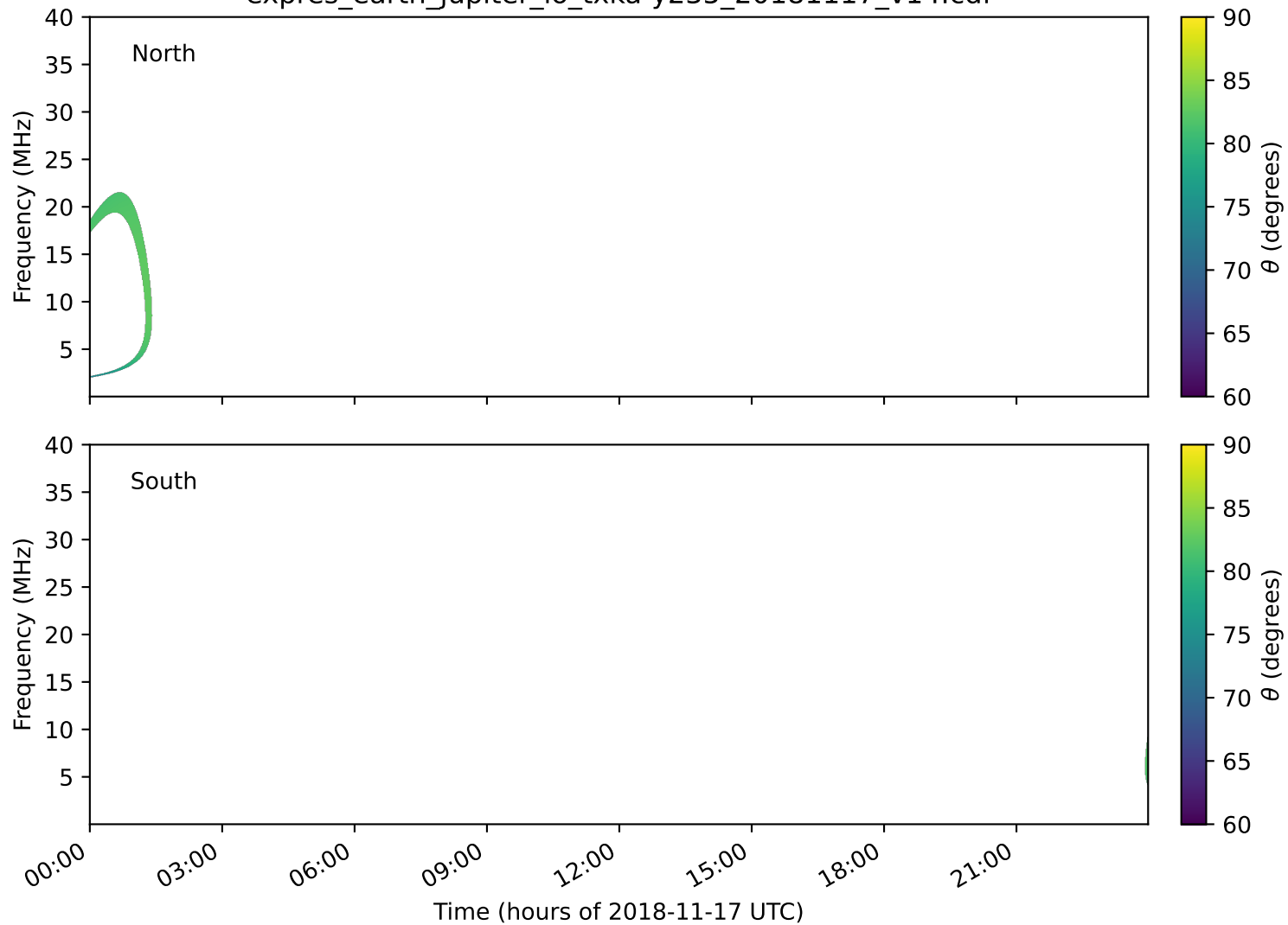
expres_earth_jupiter_io_txka-y235_20181117_v14.cdf
