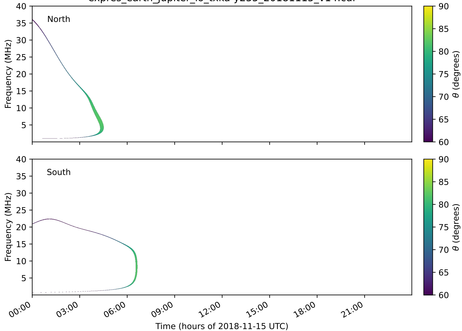
expres_earth_jupiter_io_txka-y235_20181115_v14.cdf
