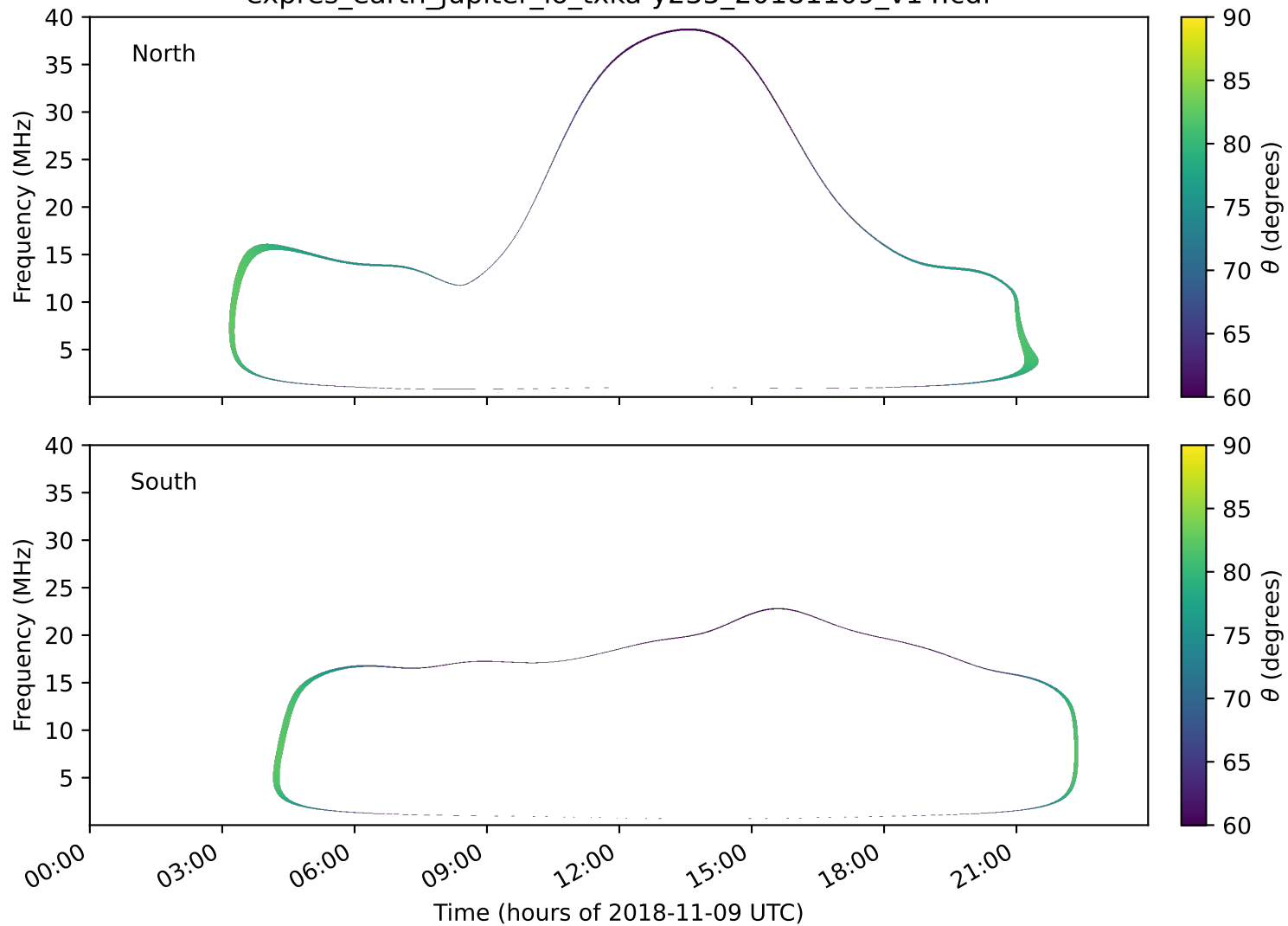
expres_earth_jupiter_io_txka-y235_20181109_v14.cdf
