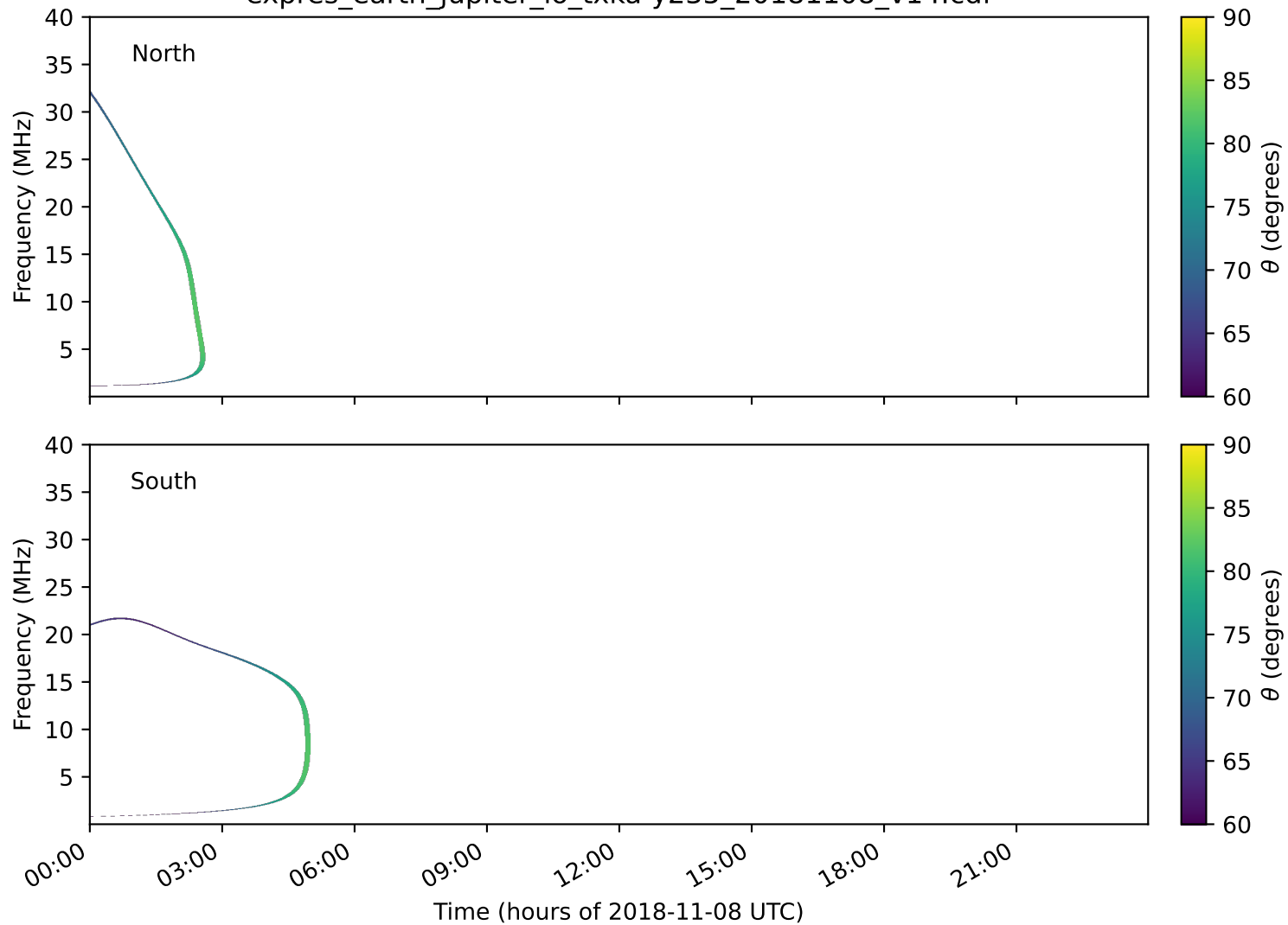
expres_earth_jupiter_io_txka-y235_20181108_v14.cdf
