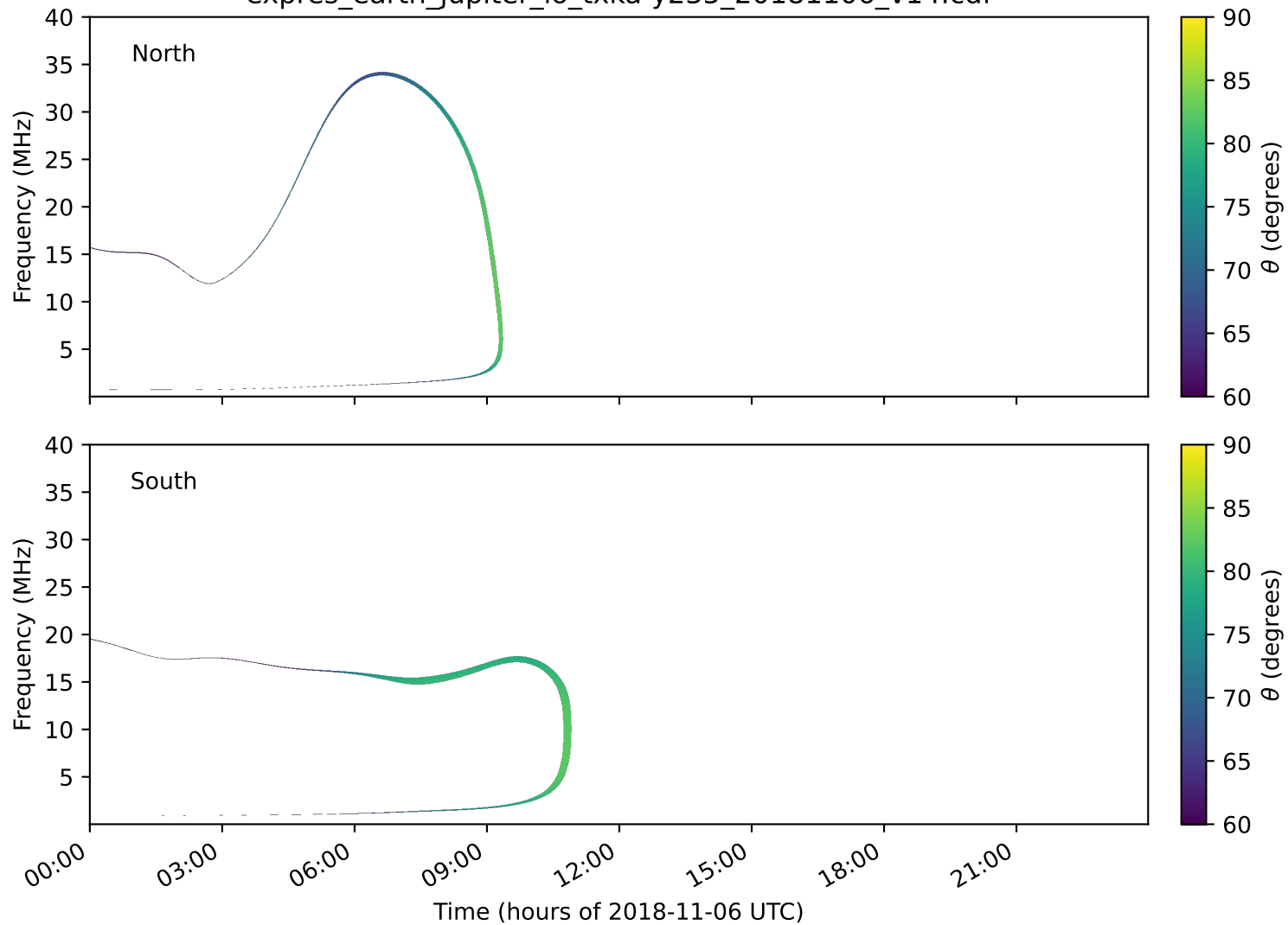
expres_earth_jupiter_io_txka-y235_20181106_v14.cdf
