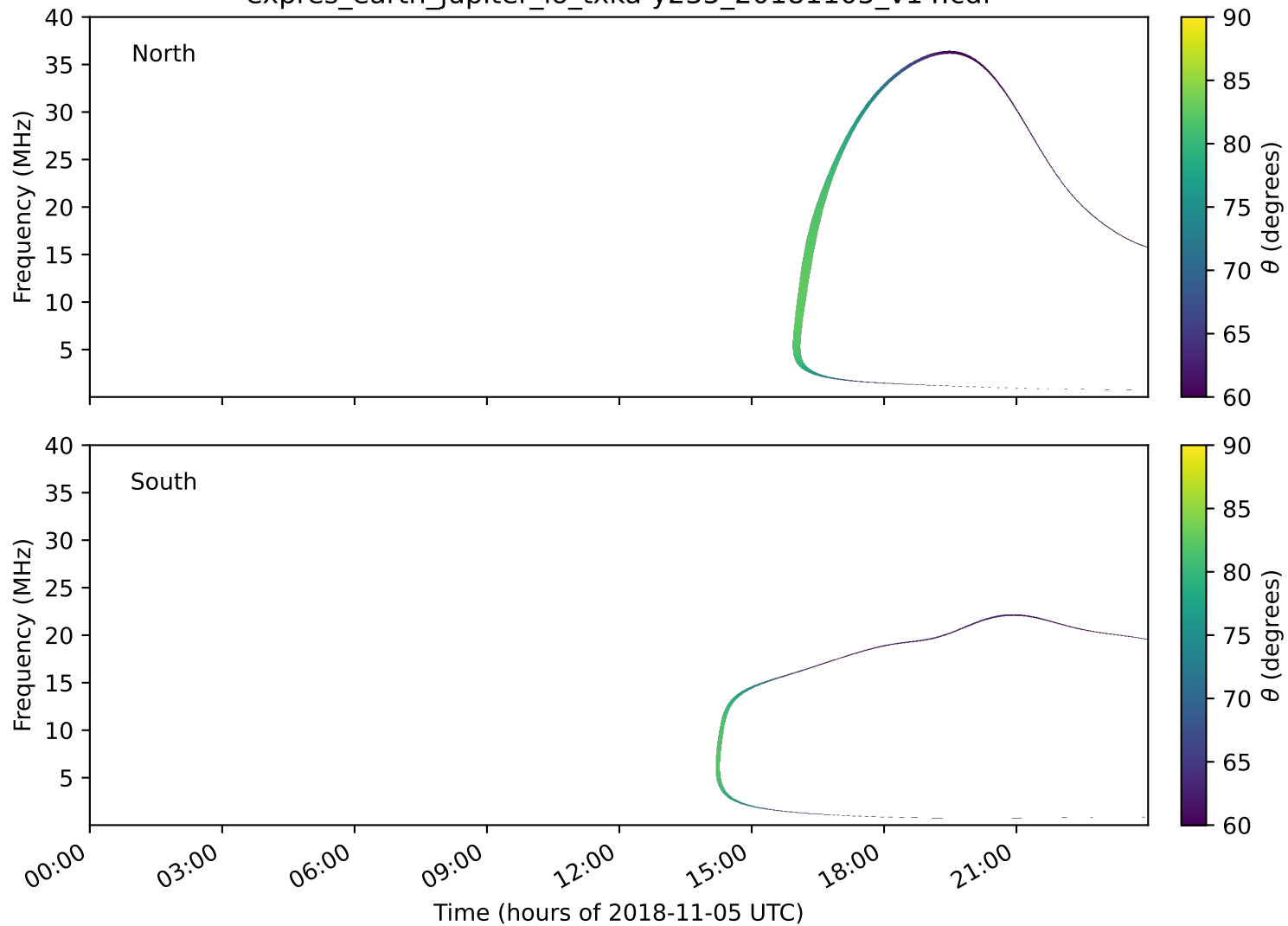
expres_earth_jupiter_io_txka-y235_20181105_v14.cdf
