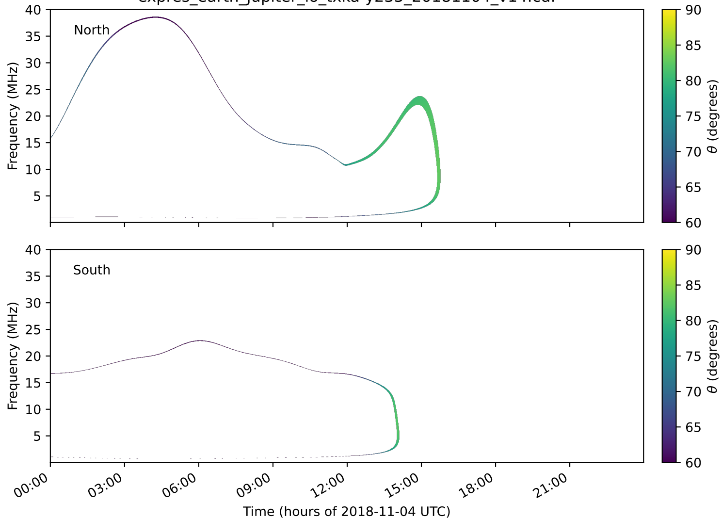
expres_earth_jupiter_io_txka-y235_20181104_v14.cdf
