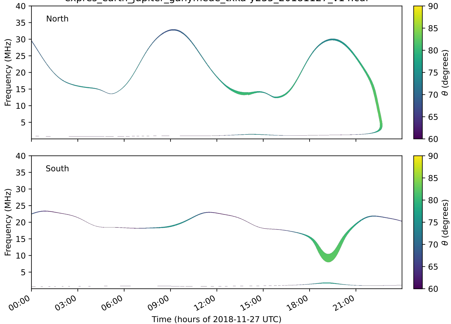
expres_earth_jupiter_ganymede_txka-y235_20181127_v14.cdf
