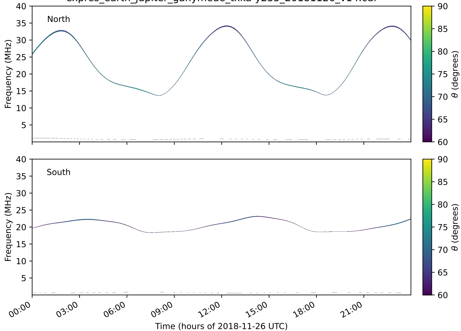
expres_earth_jupiter_ganymede_txka-y235_20181126_v14.cdf
