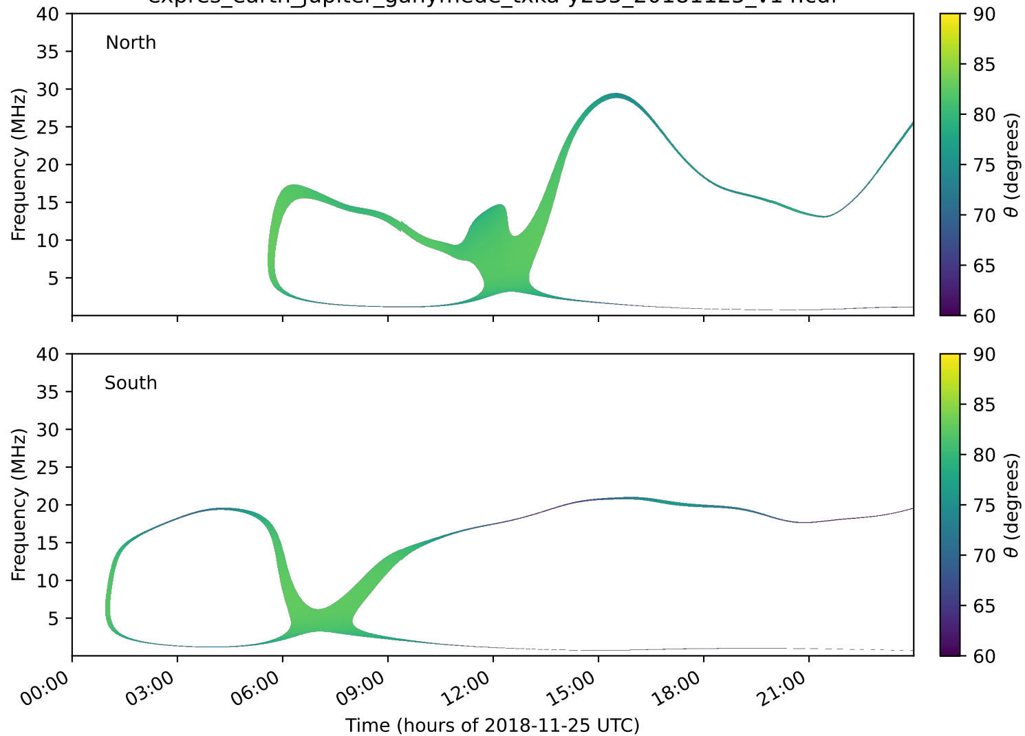
expres_earth_jupiter_ganymede_txka-y235_20181125_v14.cdf
