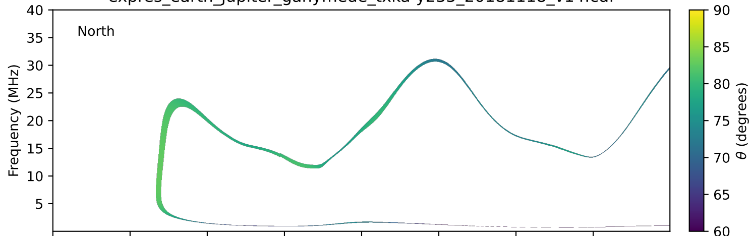
expres_earth_jupiter_ganymede_txka-y235_20181118_v14.cdf
