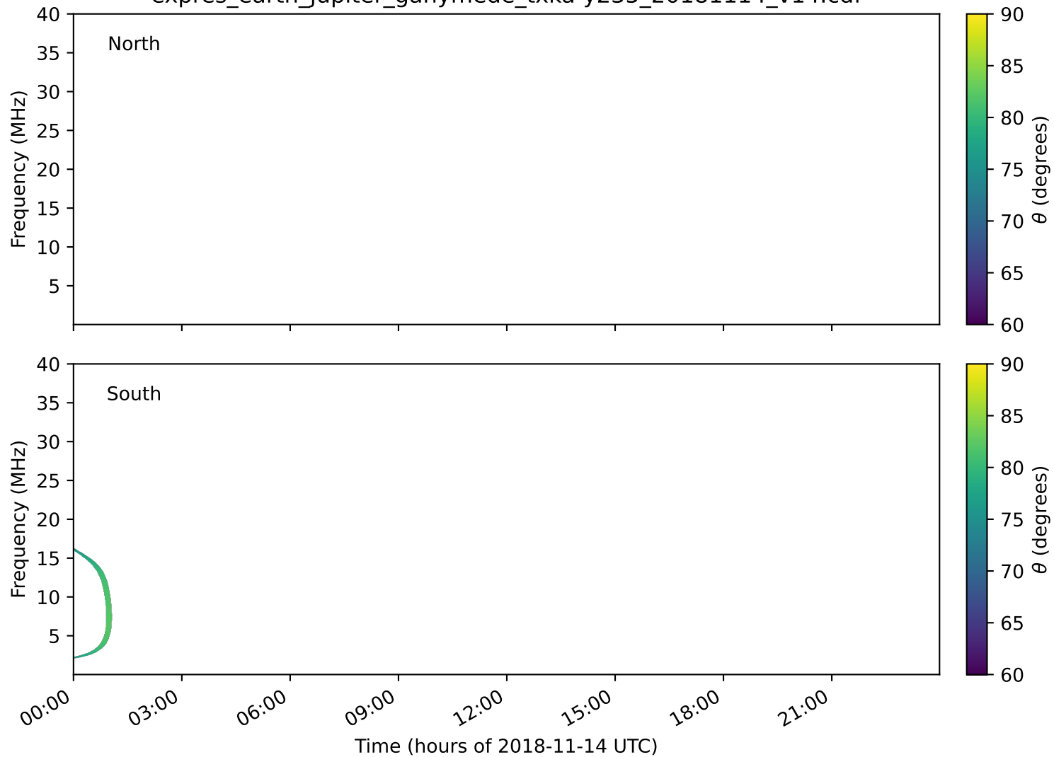
expres_earth_jupiter_ganymede_txka-y235_20181114_v14.cdf
