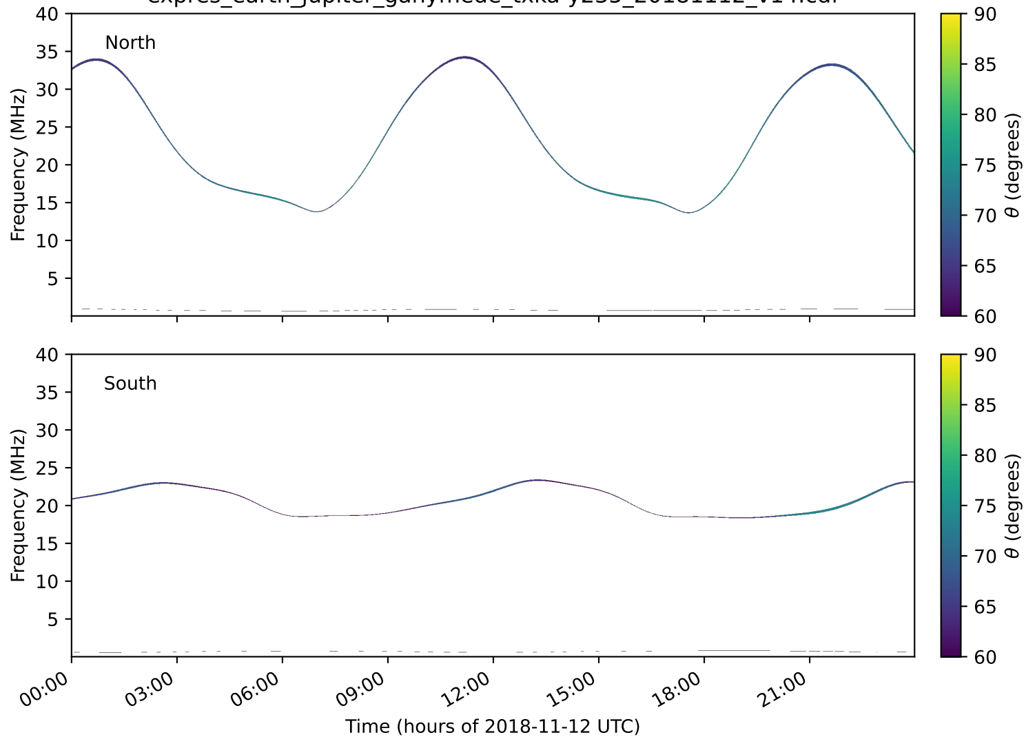
expres_earth_jupiter_ganymede_txka-y235_20181112_v14.cdf
