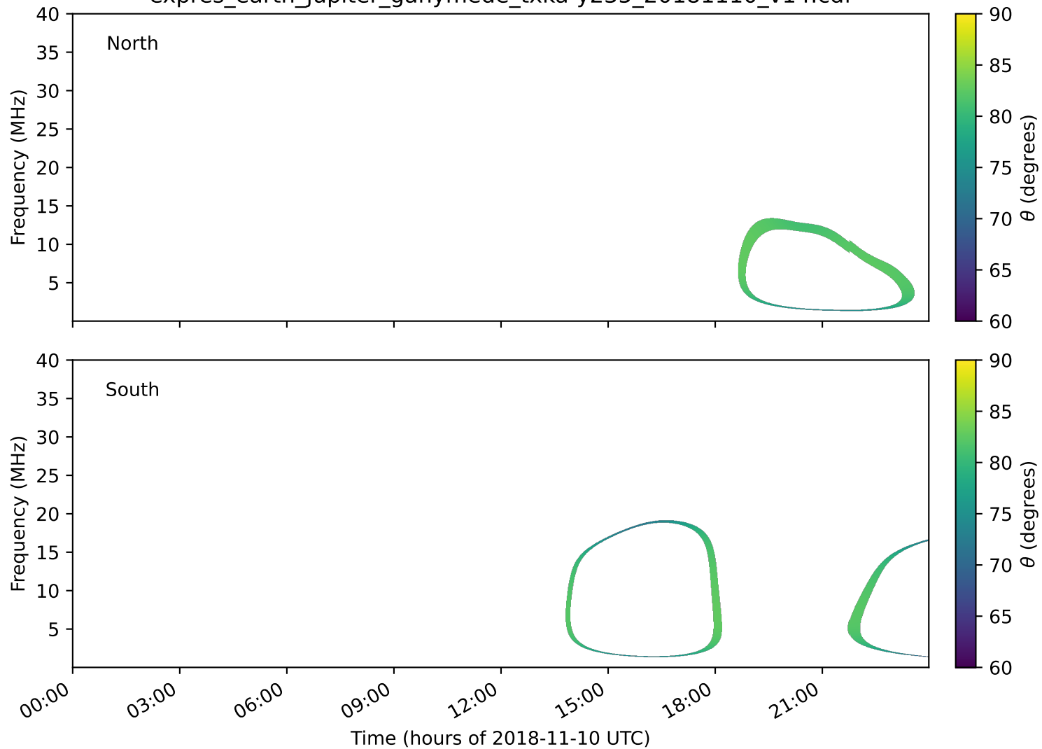
expres_earth_jupiter_ganymede_txka-y235_20181110_v14.cdf
