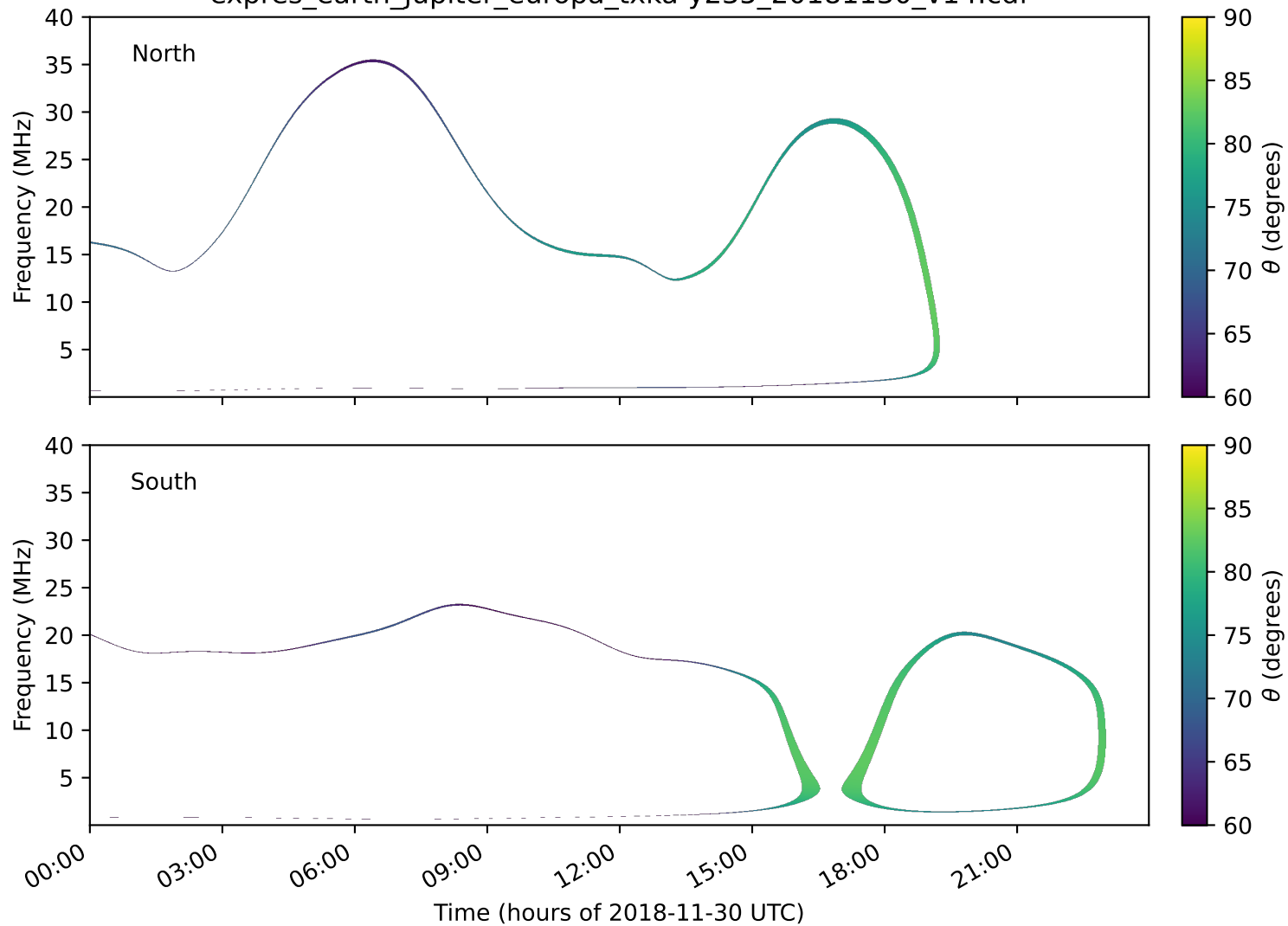
expres_earth_jupiter_europa_txka-y235_20181130_v14.cdf
