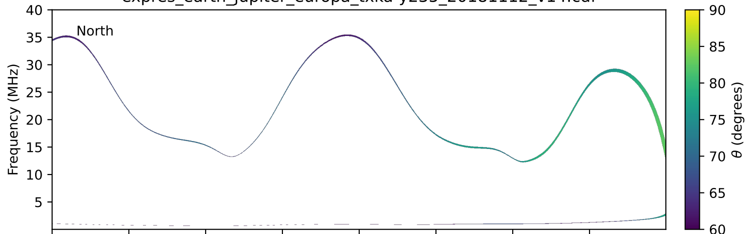
expres_earth_jupiter_europa_txka-y235_20181112_v14.cdf
