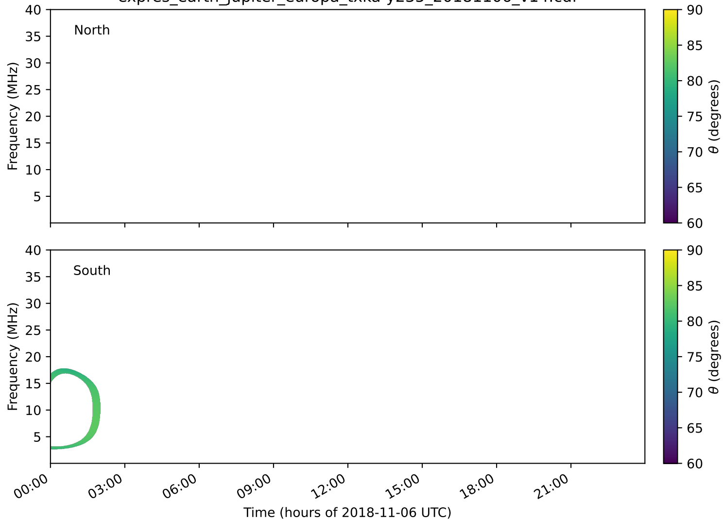
expres_earth_jupiter_europa_txka-y235_20181106_v14.cdf
