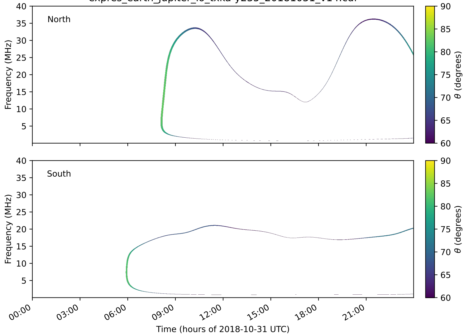
expres_earth_jupiter_io_txka-y235_20181031_v14.cdf
