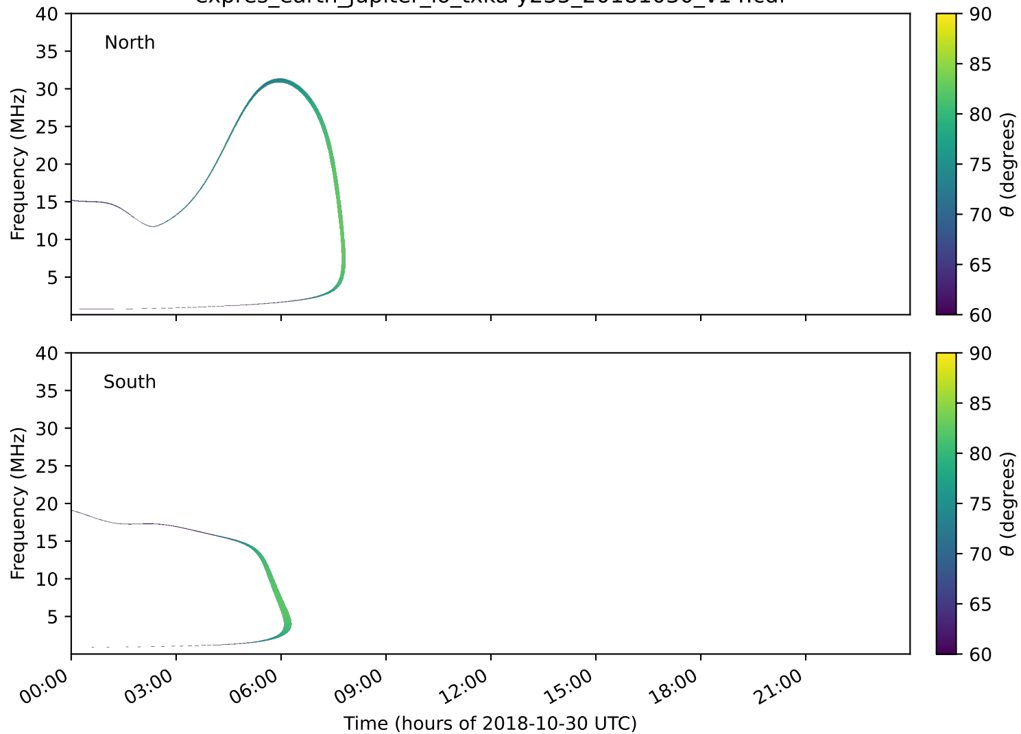
expres_earth_jupiter_io_txka-y235_20181030_v14.cdf
