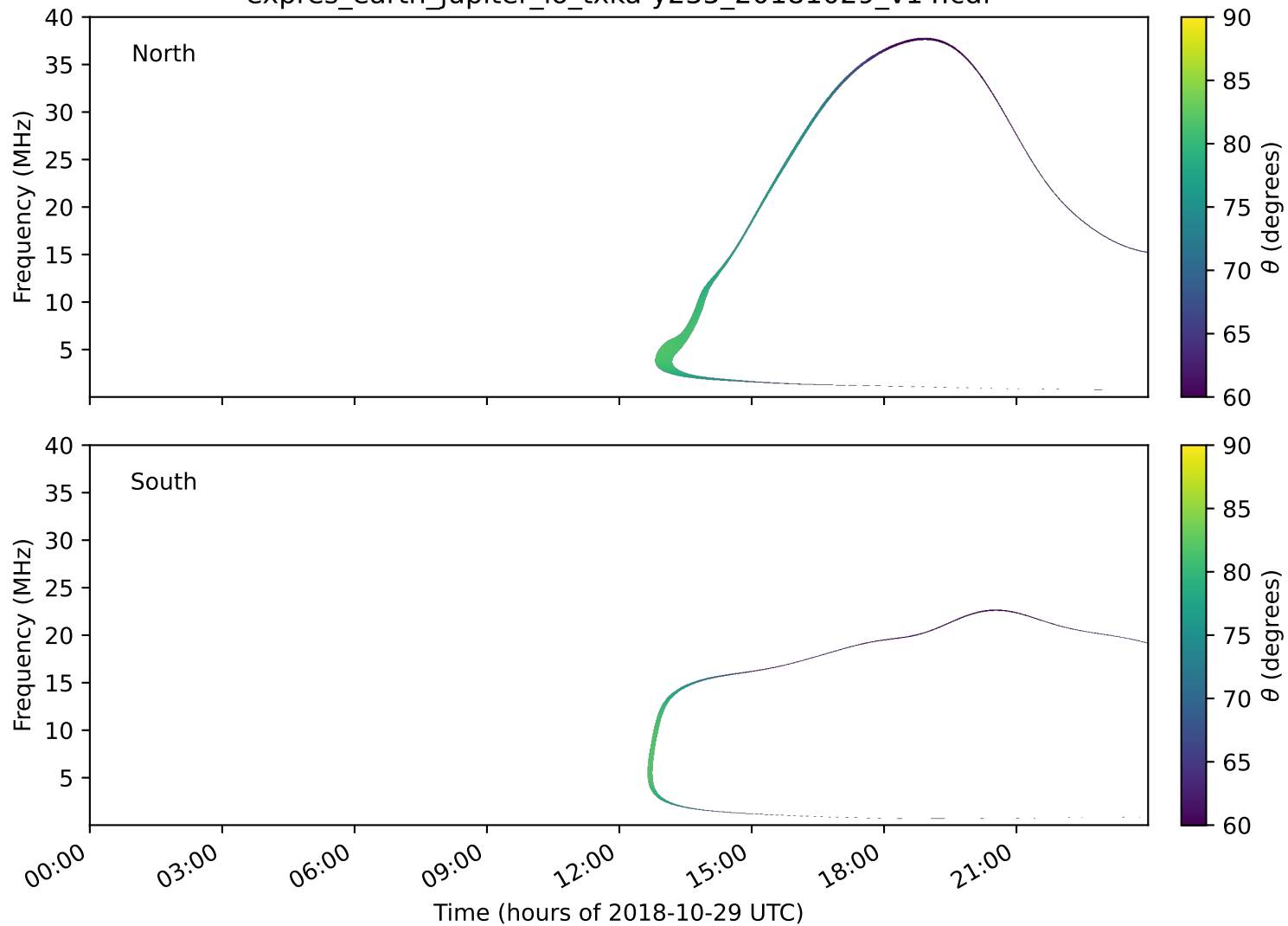
expres_earth_jupiter_io_txka-y235_20181029_v14.cdf
