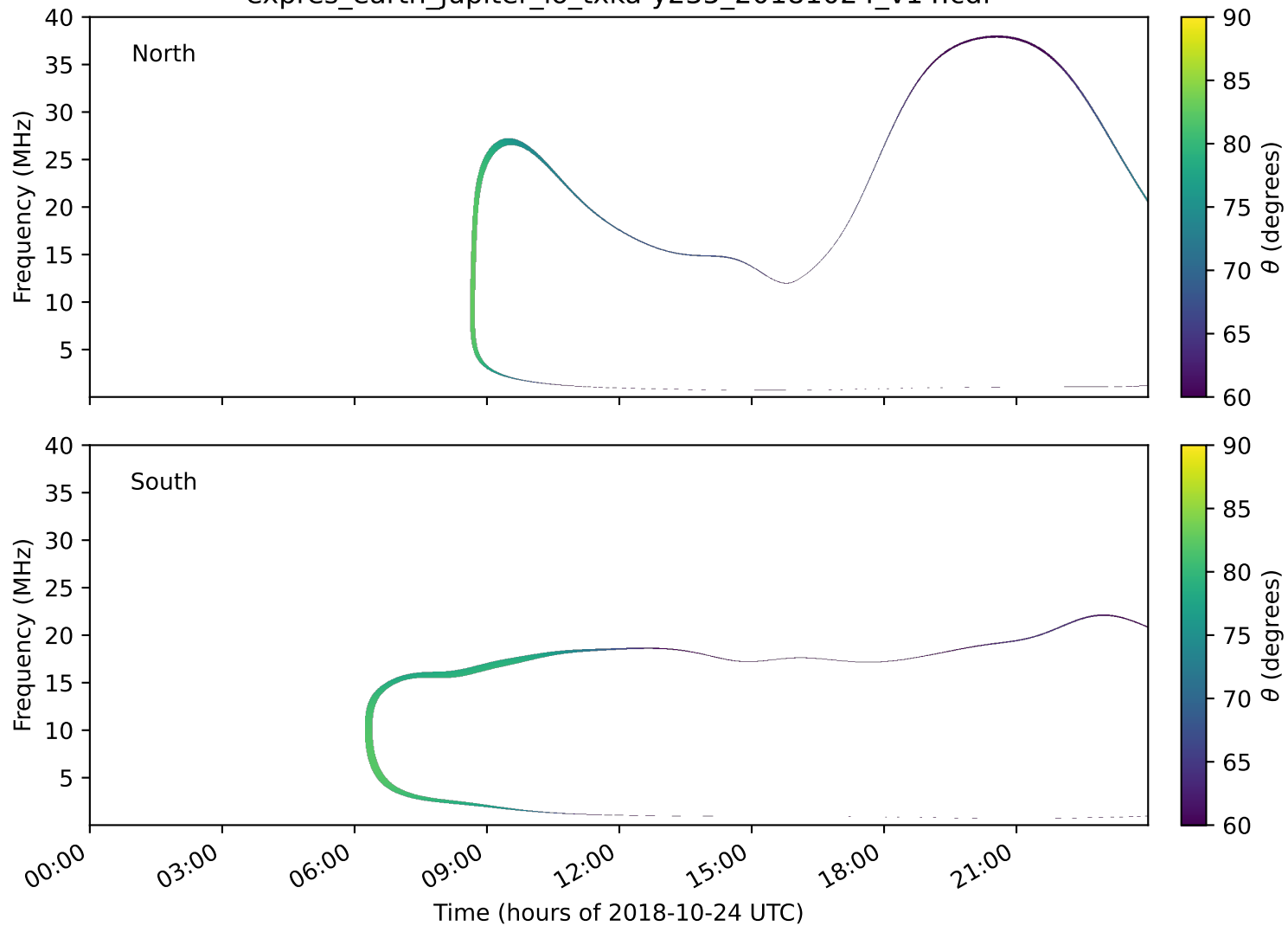
expres_earth_jupiter_io_txka-y235_20181024_v14.cdf
