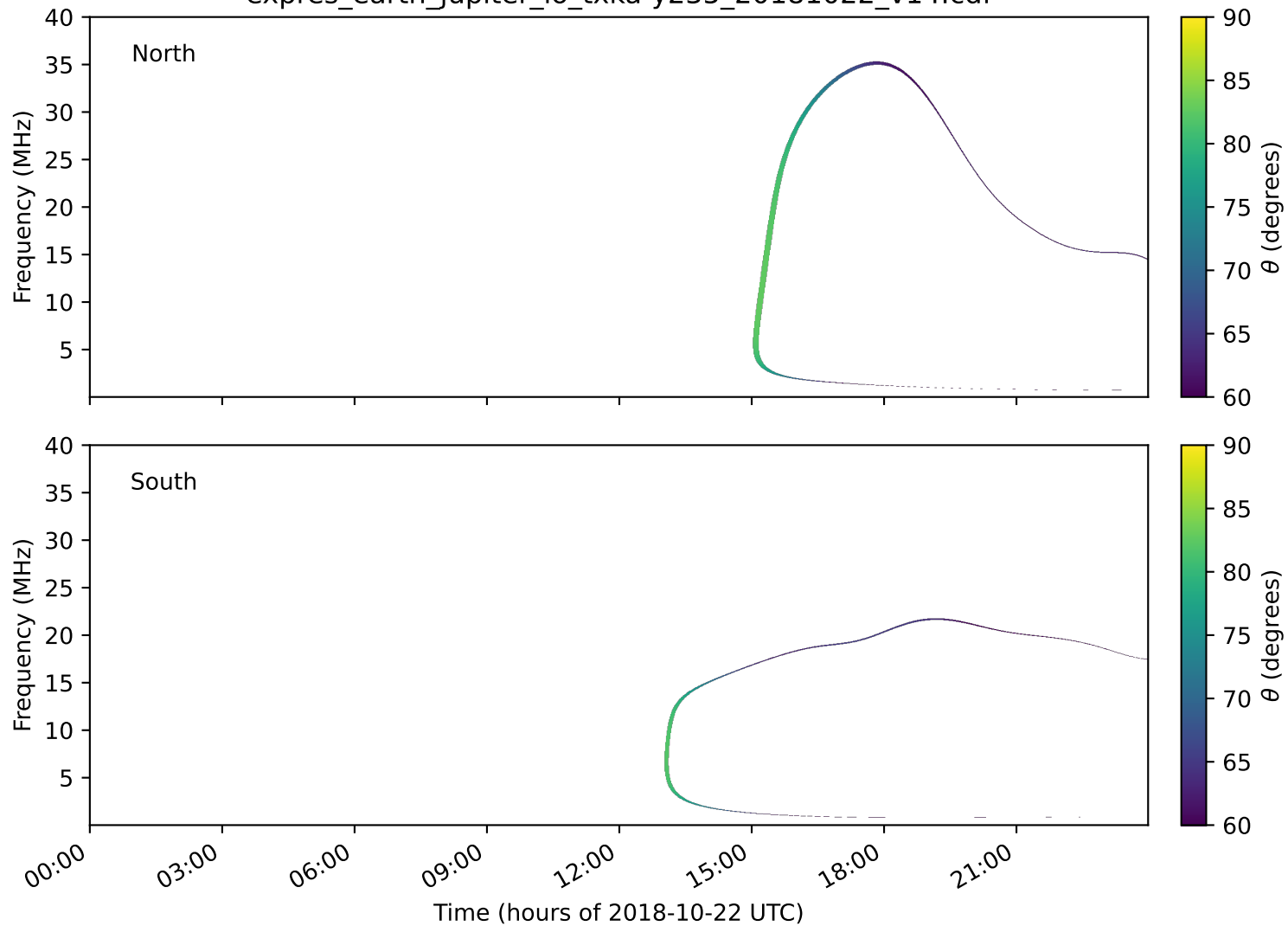
expres_earth_jupiter_io_txka-y235_20181022_v14.cdf
