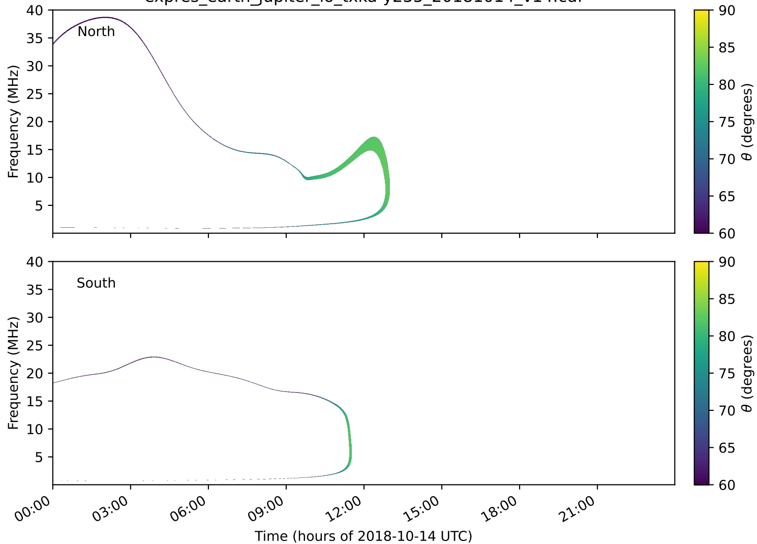
expres_earth_jupiter_io_txka-y235_20181014_v14.cdf
