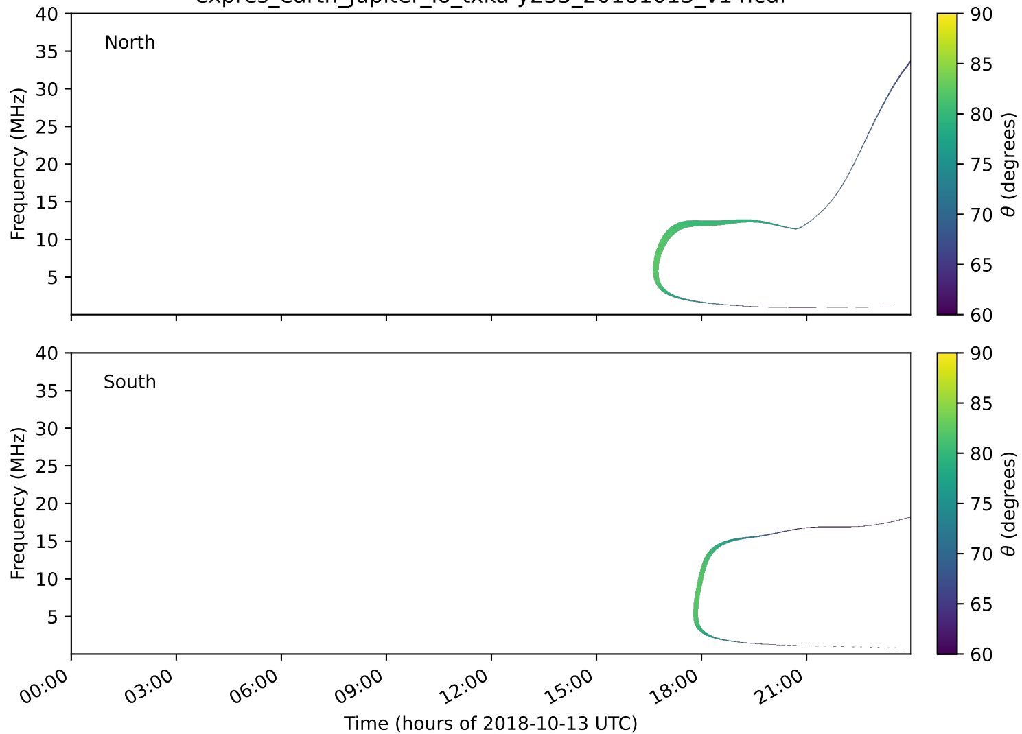
expres_earth_jupiter_io_txka-y235_20181013_v14.cdf
