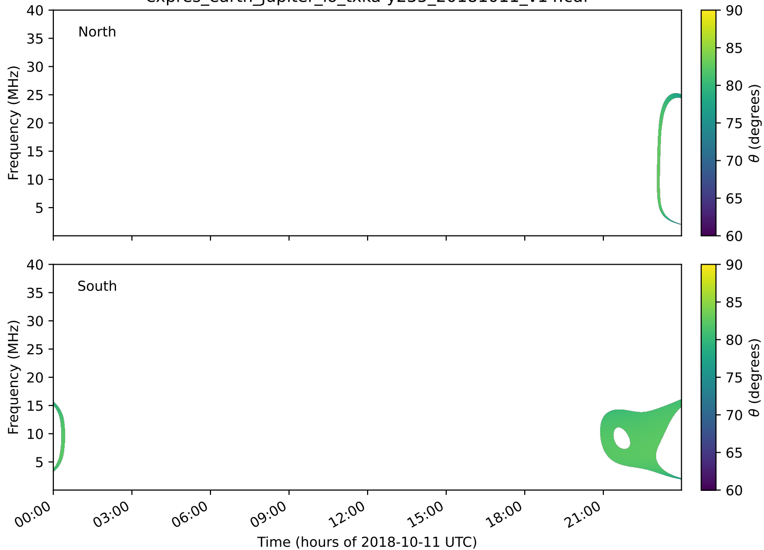
expres_earth_jupiter_io_txka-y235_20181011_v14.cdf
