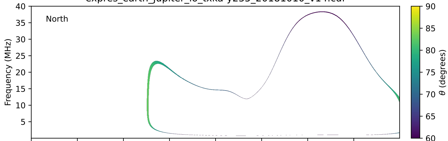
expres_earth_jupiter_io_txka-y235_20181010_v14.cdf
