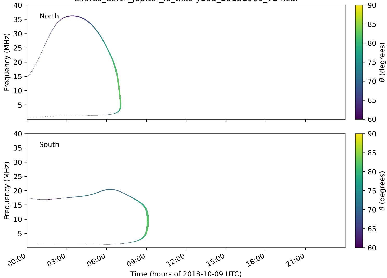
expres_earth_jupiter_io_txka-y235_20181009_v14.cdf
