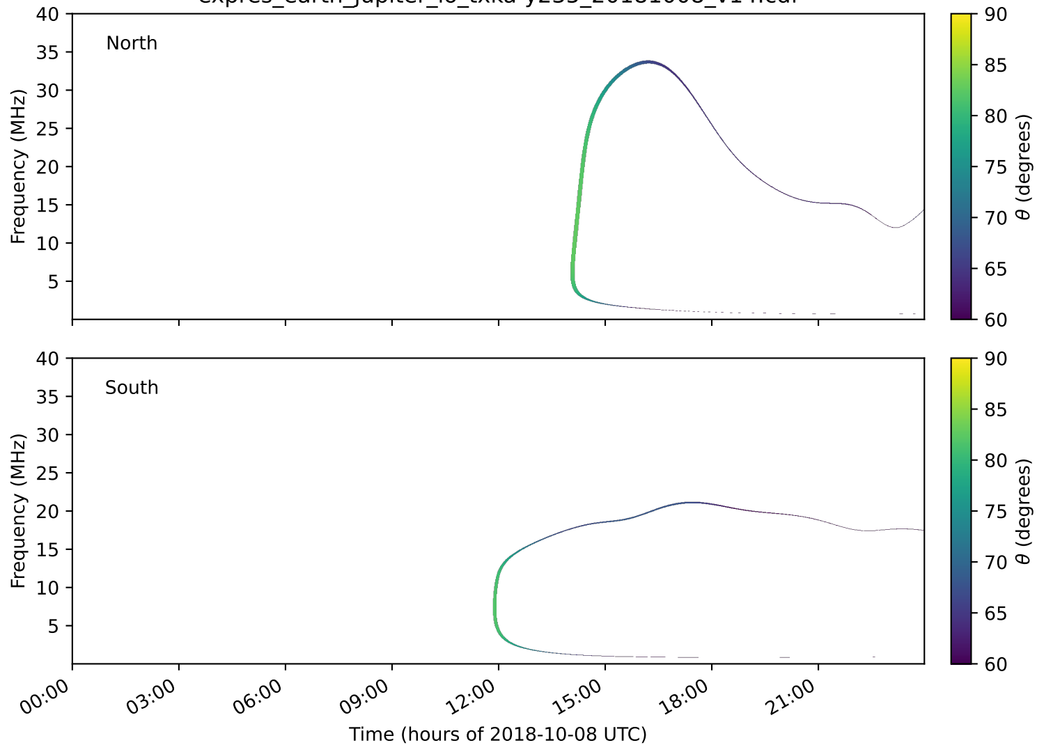
expres_earth_jupiter_io_txka-y235_20181008_v14.cdf
