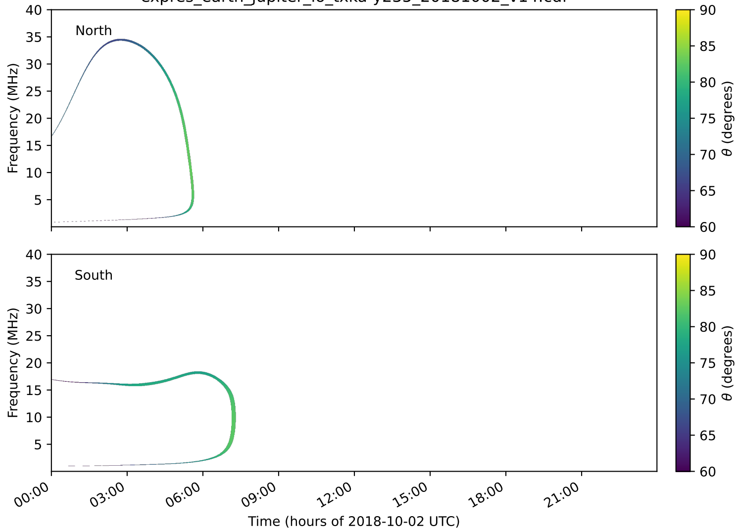
expres_earth_jupiter_io_txka-y235_20181002_v14.cdf
