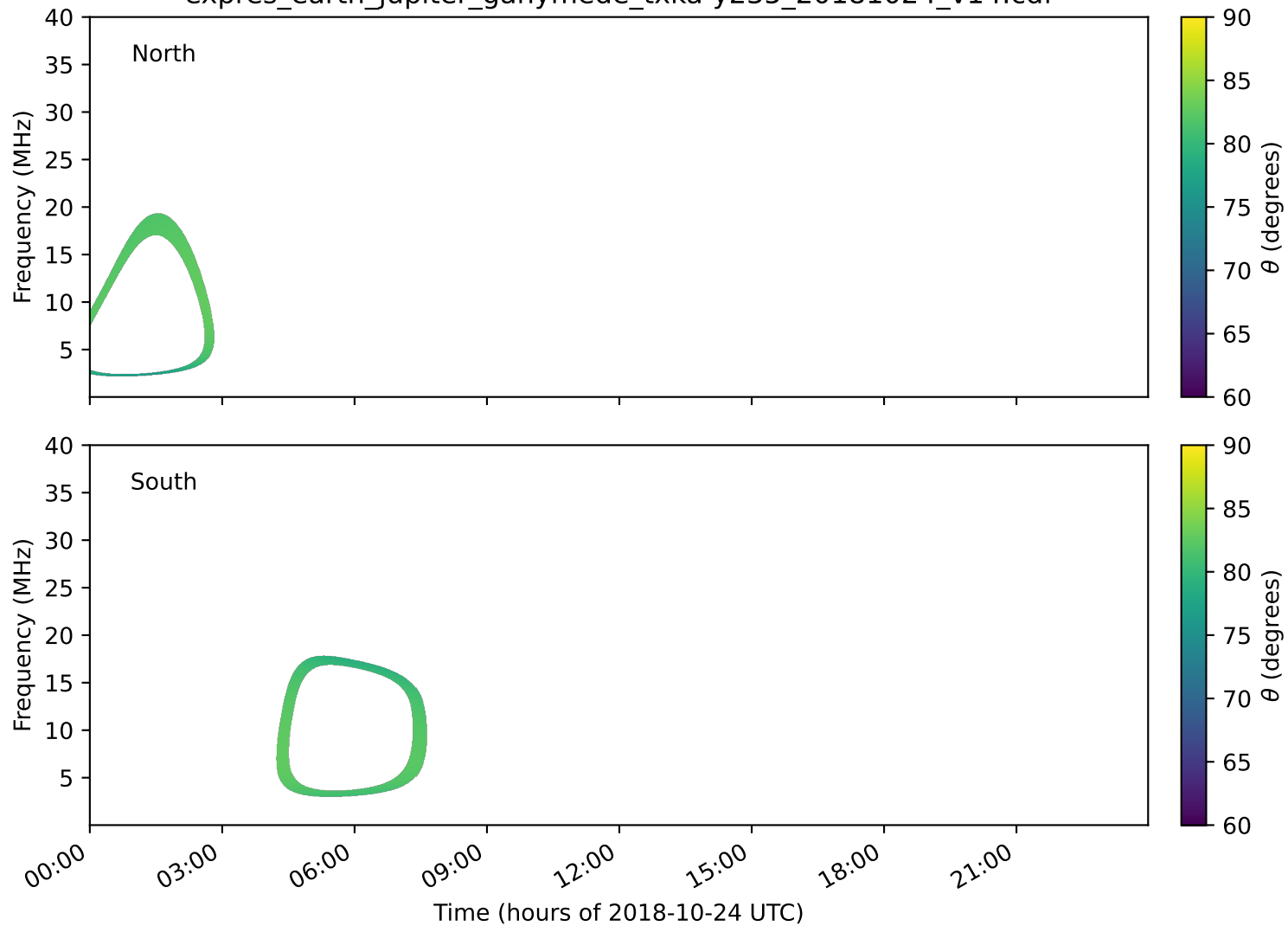
expres_earth_jupiter_ganymede_txka-y235_20181024_v14.cdf
