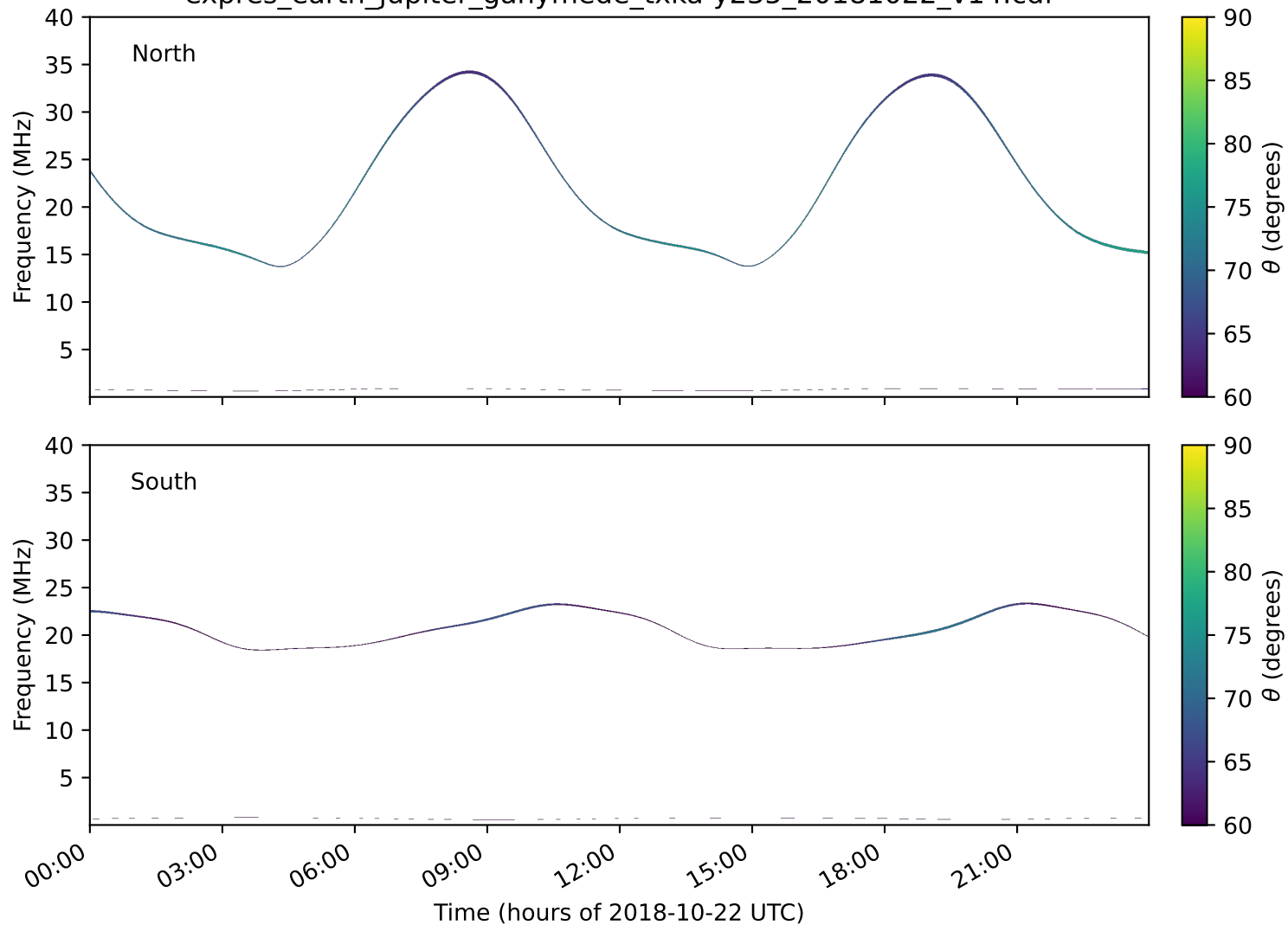
expres_earth_jupiter_ganymede_txka-y235_20181022_v14.cdf
