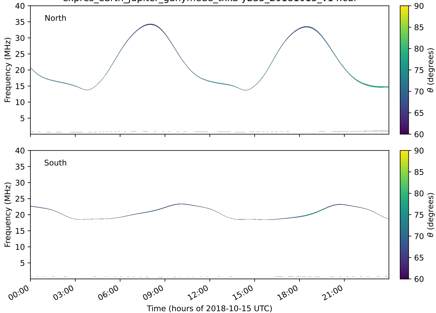
expres_earth_jupiter_ganymede_txka-y235_20181015_v14.cdf
